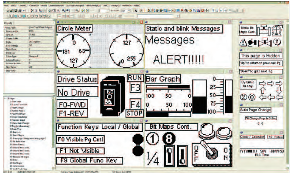
ELCSoftGP—Editing Environment
