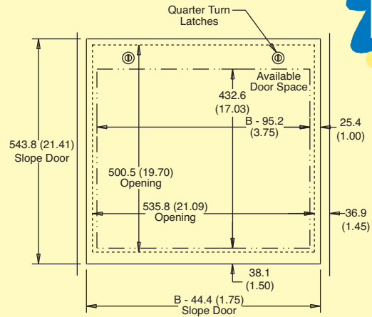
View B-B
