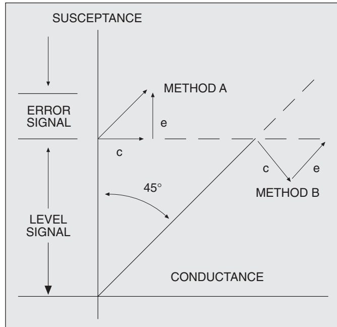
Admittance Vector Diagram Figure 6
