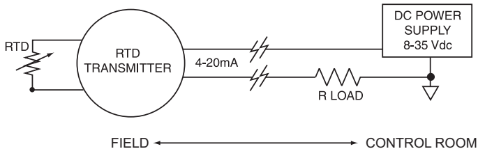
Figure 1-1 RTD Transmitter
