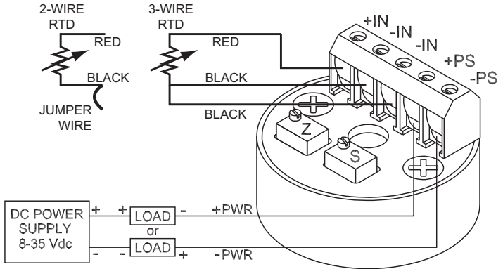
Figure 2-2 Wiring Diagram for RTD Transmitter
