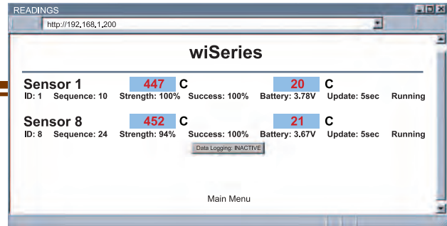
Temperature Readings of up to 8 Sensors
