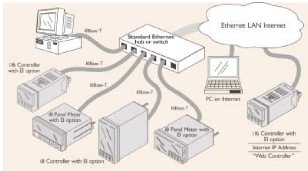
Fig 2 Direct connection to Ethernet LAN or Internet
