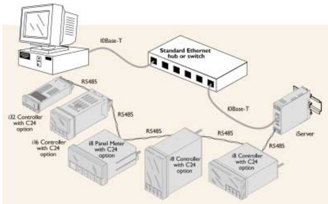
Fig 3 Integration of server controller hub for up to 32 devices
