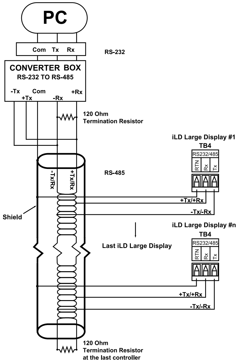
Figure 3.3 Multipoint, Half-Duplex RS-485 wiring
