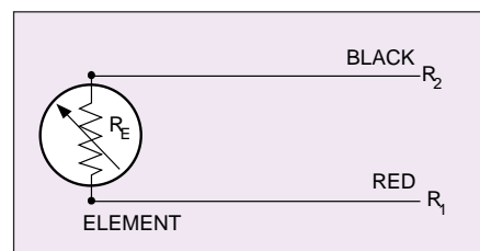
FIGURE 2. 2-WIRE CONFIGURATION (STYLE 1)
