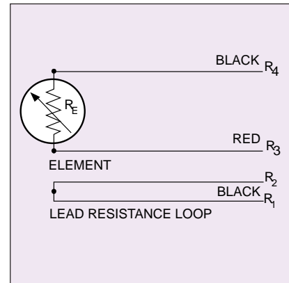
FIGURE 5. 2-WIRE CONFIGURATION PLUS LOOP (STYLE 4)
